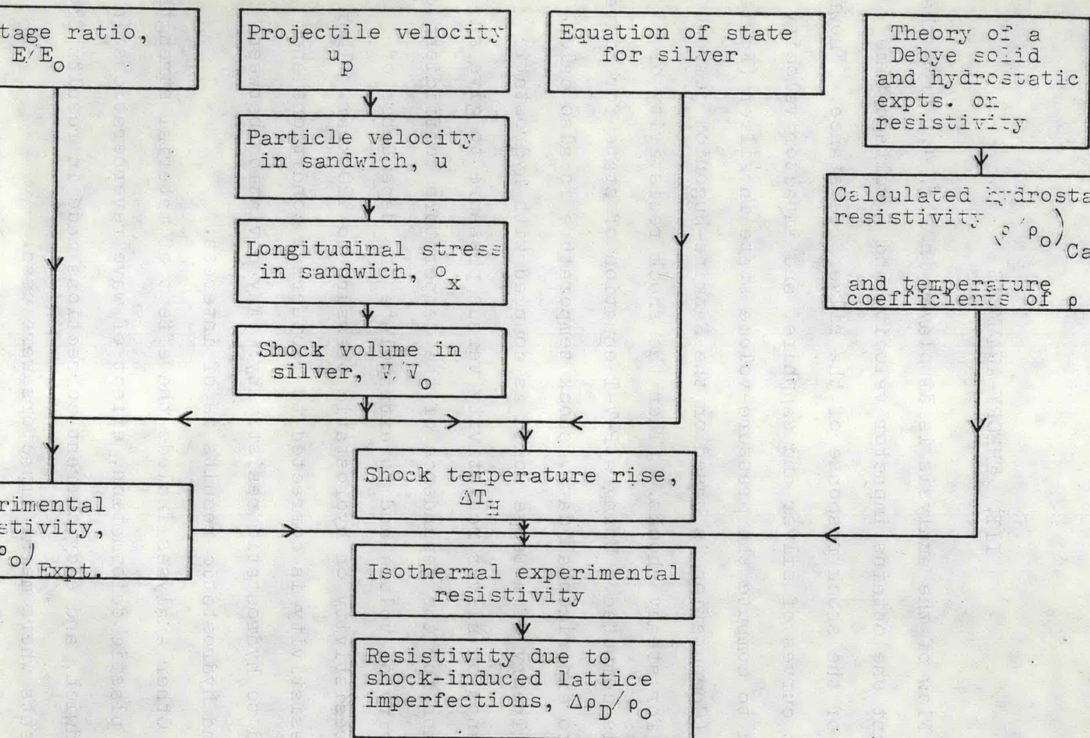
Fig. 4. Analysis flow chart.
